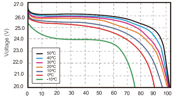
DISCHARGE CAPACITY at VARIOUS TEMPERATURES DISCHARGE @0.2 C
