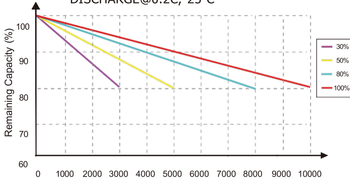
CYCLE LIFE vs. DEPTH OF DISCHARGE(DOD) DISCHARGE@0.2C, 25 C
